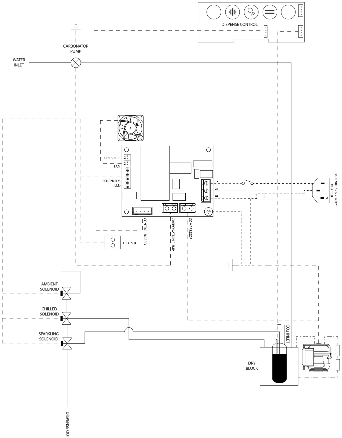
Chilled, Ambient & Hot Circuit Schematic
