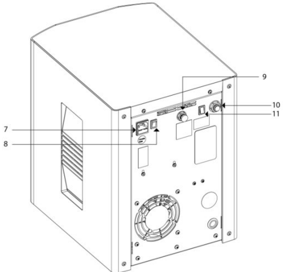
1. Unit Lid, 2. Side Panel, 3. Carry Handle, 4. Control Panel, 5. Dispense Outlet, 6. Drip Tray, 7. Power Connection, 8. On/Off Switch, 9. CO2 Inlet*, 10. Water Inlet, 11. Hot Tank Switch
