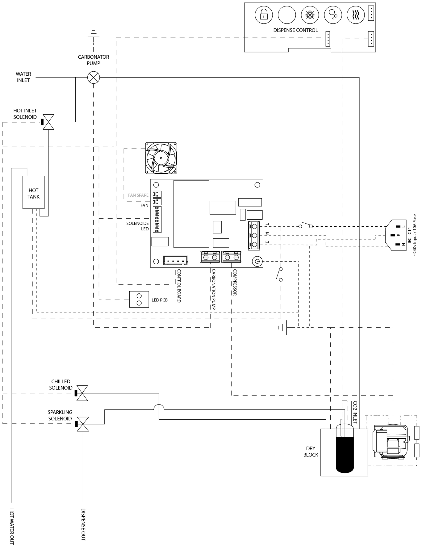
Water Pathway - Chilled & Ambient
